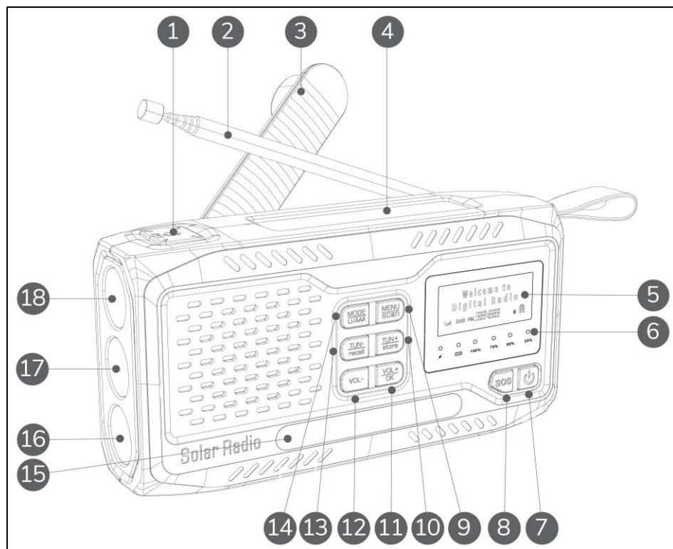
Figure 1: Front view.
