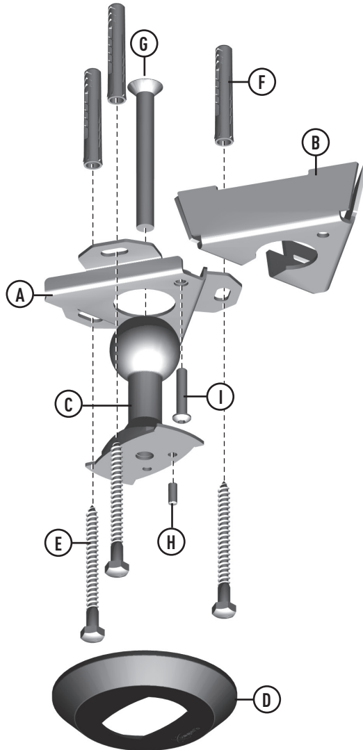
PUC 1040 Ceiling plate
