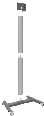
DIVISIBLE DISPLAY TROLLEY MAX. 55 INCH, 30 KG
