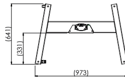
DIVISIBLE DISPLAY TROLLEY MAX. 55 INCH, 30 KG
